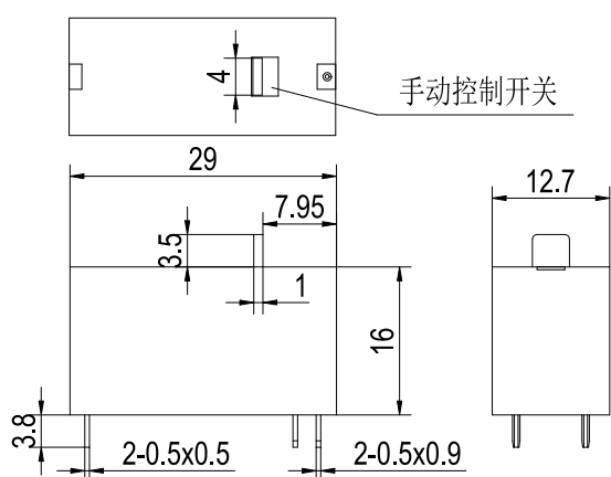
1A3/1B3(双线圈)
