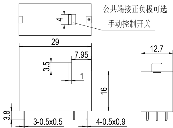
1A3/1B3(单线圈)
