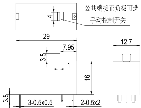
1A2/1B2(单线圈)
