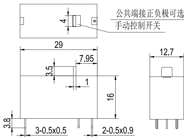
1A6/1B6(单线圈)
